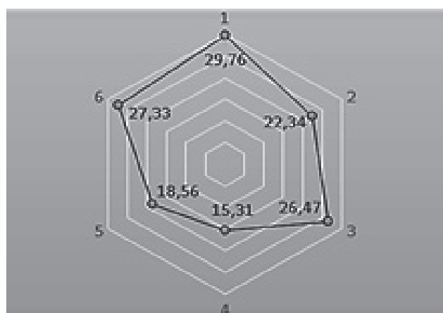
Figure 8. Example of an individual model calculated on the basis of sigma estimates T
